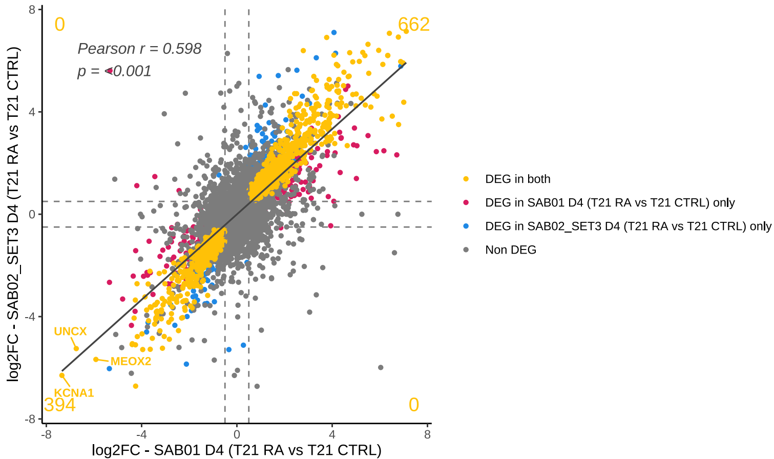
Comparison between SAB01 D4 (T21 RA vs T21 CTRL) and SAB02_SET3 D4 (T21 RA vs T21 CTRL)
